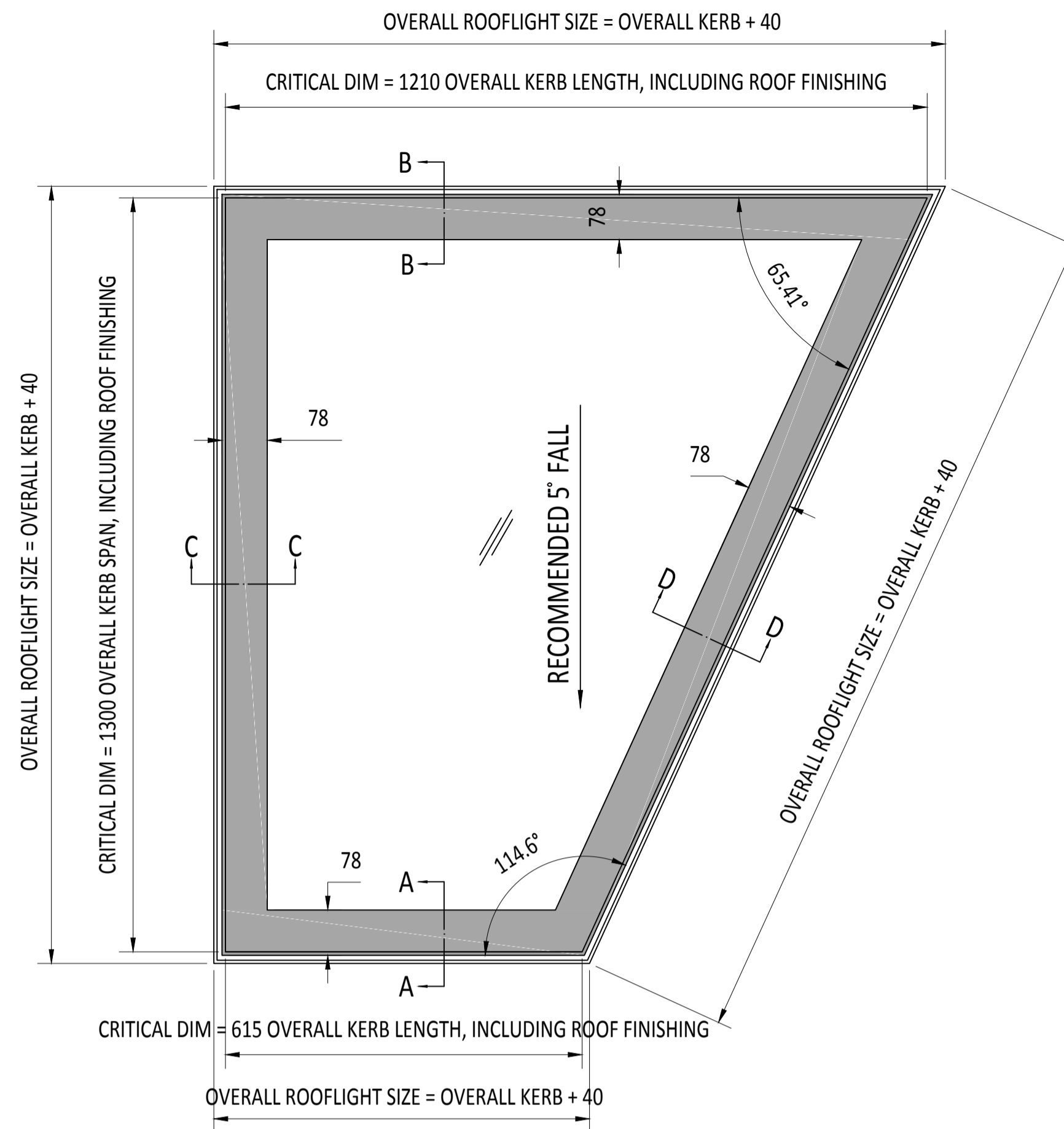
PLAN VIEW True view on slope
